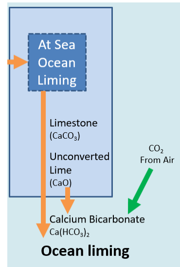
Figure 4: Ocean Liming with used sorbent
