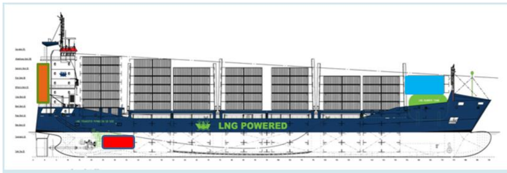
Figure 2: The system configuration on a ship showing relative equipment sizes
