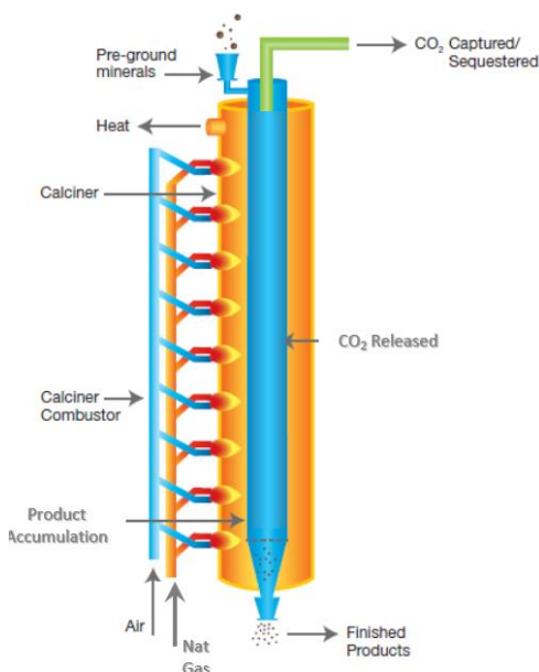
Figure 3: Diagram of the LEILAC Direct separation calciner
