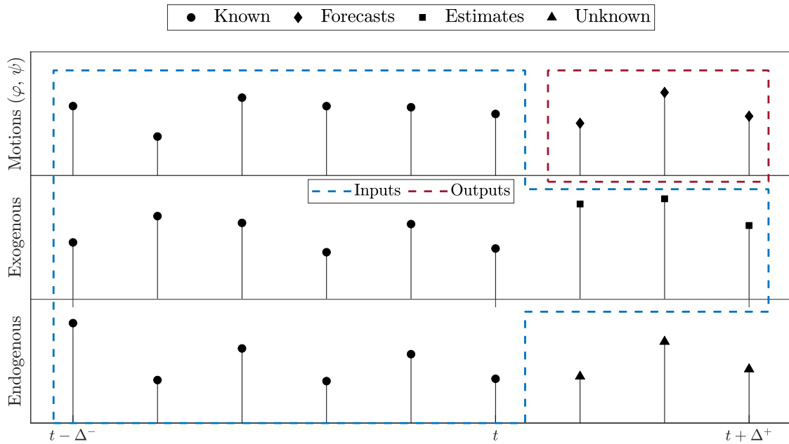
Figure 3: The short-term motions forecasting framework with the window of historical data in the period [t - \Delta^-, t] , the forecast horizon(s) up to t + \Delta^+ , and estimations of some features during the period (t, t + \Delta^+] .
