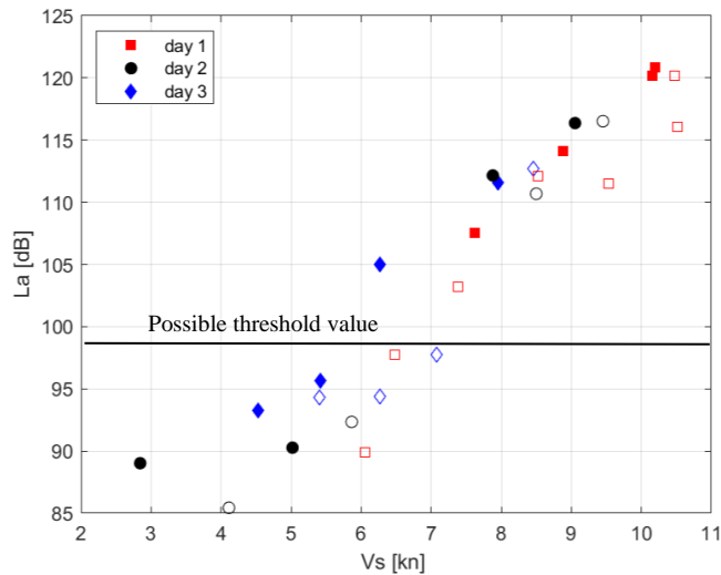
Figure 16: Acceleration level per 1/3 octave band with centre frequency of 1 kHz. Open symbols are trials in the eastwards direction and closed symbols are in westwards direction.
