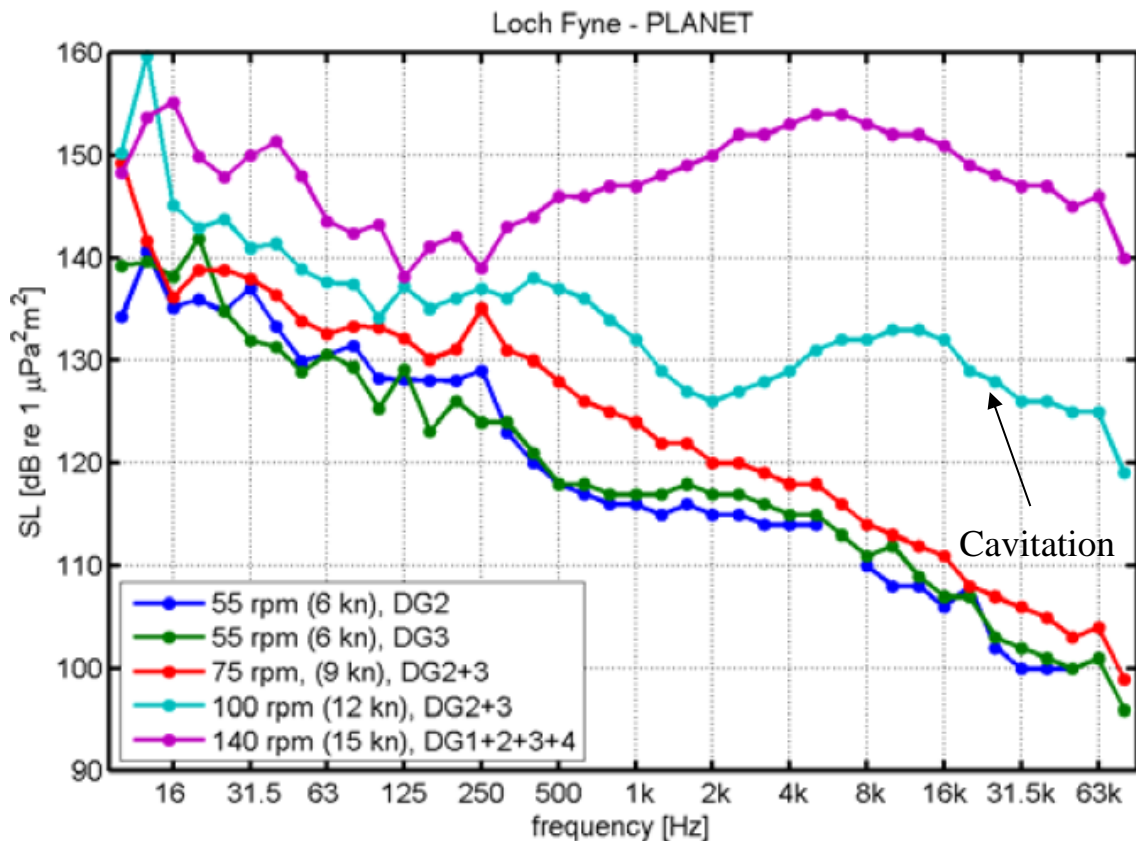
Figure 9 : Acoustic measurement of RV Planet (de Jong, 2016)
