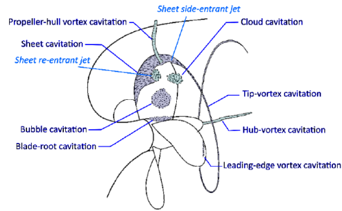
Figure 8 Types of cavitation [1]
