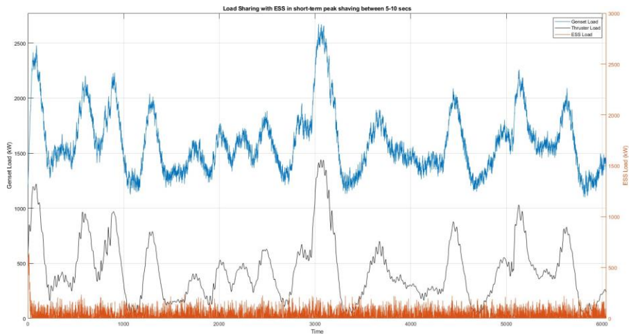
Figure 8: ESS load profile with genset in short-term peak shaving
