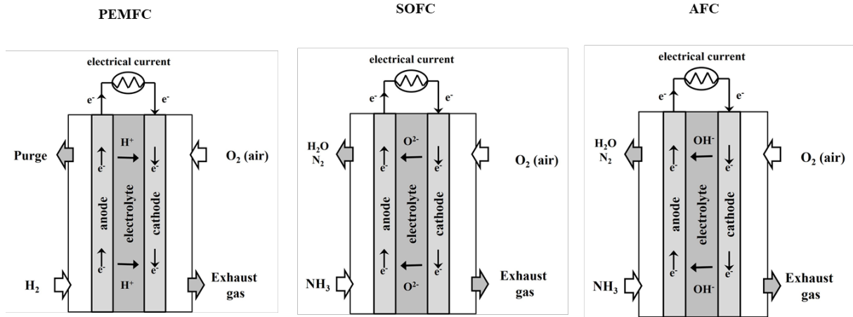
Figure 1: PEMFC, SOFC and AFC working schemes
