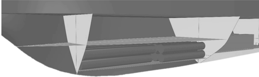
Figure 5: Ammonia storage tanks arrangement
