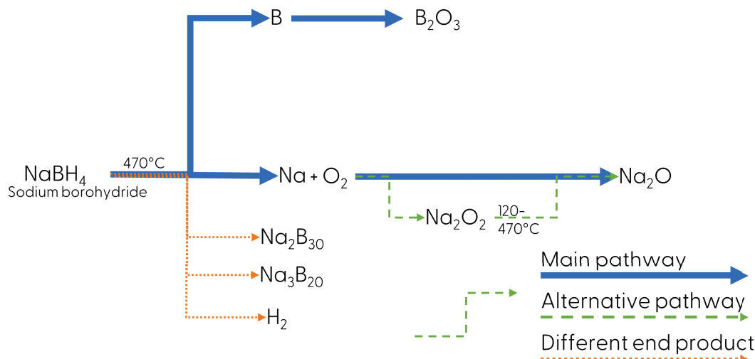
Figure 3: Reactions of sodium borohydride in heat
