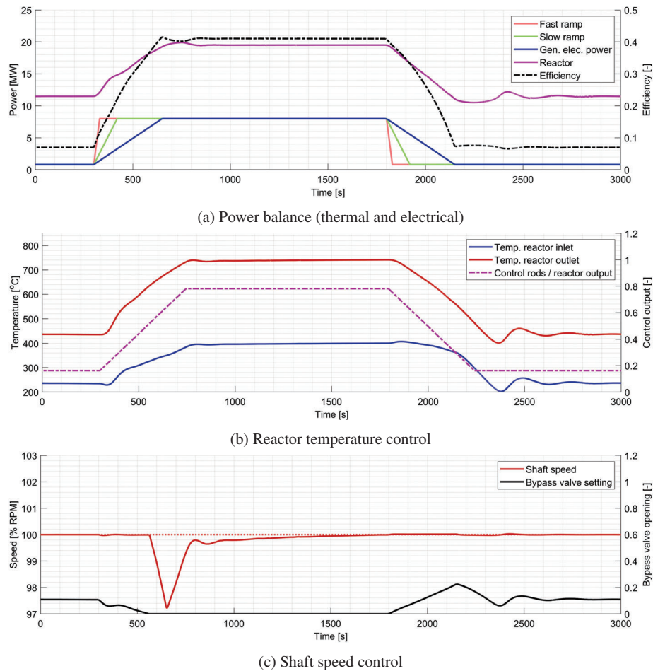
Figure 8: Simulation results scenario 1, reactor limitations
