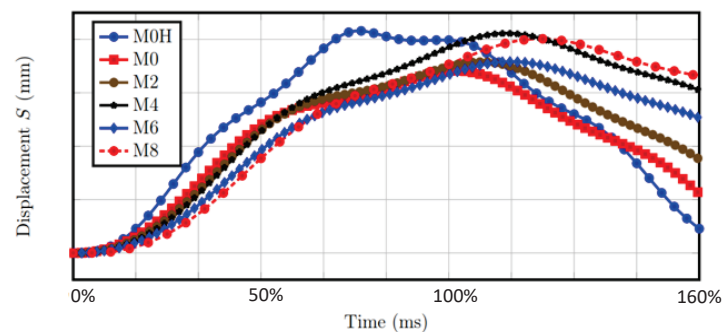
Figure 5: Displacement Profiles Produced by the Drop Test Rig with Varying Mass
