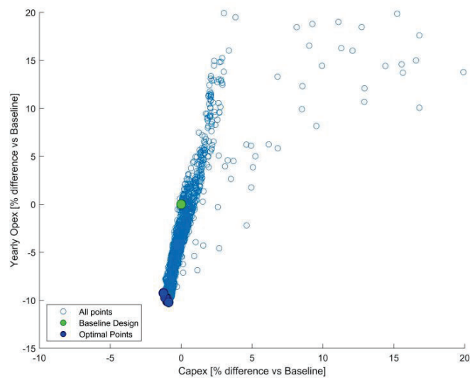
Figure 9: Optimization of EMS setpoints
