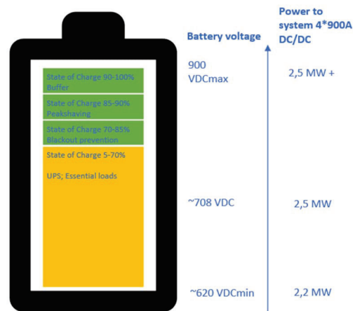
Figure 4 – Example for visual representation of Battery usage, Battery voltage and available power to the system (total for vessel).
