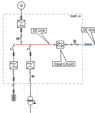
Figure 5: Notional SLD detail for a combatant damage zone BESS integration
