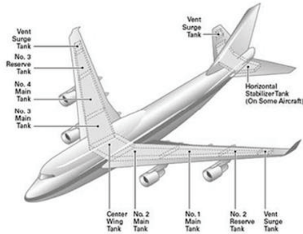
Figure 2 – 747-400 Wing-Integrated Fuel Tank Arrangement
